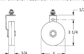
ROTARY BRACKET ASSEMBLY WITH MOUNTING STUD
